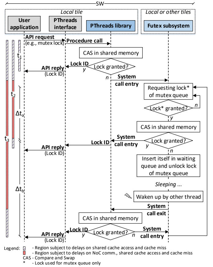
Fig. 3. Synchronization control flow employed on Linux-only based solution.
