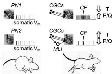
Fig. 2. Hypothesis on the role of feed-forward inhibition in determining the \text{Ca}^{2+} source associated with the CF input. On the left, two PNs (PN1 and PN2) firing at the same frequency when the mouse is at rest; on the right, PN1 increases the firing frequency with movement following excitation provided by CGC inputs while PN2 decreases the firing frequency following a dominance of MLI feed-forward inhibition; PN1 would favour activation of P/Q channels following a CF input while PN2 would favour activation of T channels following a CF input.
