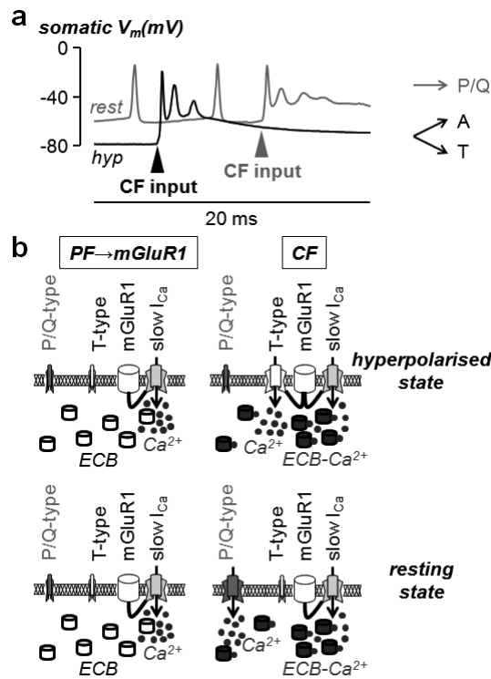
Fig. 1. \text{Ca}^{2+} sources responsible for \text{Ca}^{2+} transients associated with CF-EPSPs and mechanisms underlying supralinear amplification. a Example of CF Somatic V_m associated with CF inputs at initial hyperpolarised V_m (black trace), activating T and A channels, and at resting V_m (gray trace), activating P/Q channels. b At both states, the slow \text{Ca}^{2+} current ( I_{\text{Ca}} ) gated by mGluR1 activation following PF activity saturates the ECB amplifying the CF \text{Ca}^{2+} transient. At the hyperpolarised state (top), this mechanism combines with the co-localised mGluR1-dependent potentiation of T-type VGCCs activated by the CF. At the resting state (bottom), this mechanism combines with the boosted CF activation of P/Q-type VGCCs, but the two mechanisms are not co-localised.
