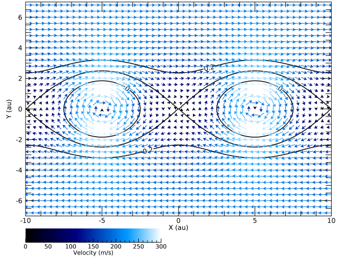
Figure 7. Velocity field in a periodic inviscid vortex sheet according to Corcos & Sherman (1976). Some of the streamlines, corresponding to the stream function values \Psi = 0, 0.1, and 0.2 times the maximum, are shown. The cat’s eyes are outlined by the contour 0.1 .
