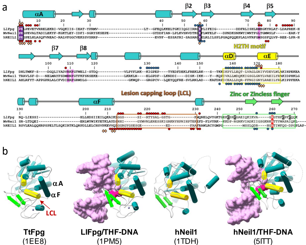
Figure S11. Structures of LIFpg, MvNei1 and hNeil1 (a) Primary structure alignment based on 3D-structures The indicated \alpha -helices (cylinders) and \beta -strands (arrows) are from LIFpg (observed in 1PM5). P1, E2 and K57 catalytic residues are boxed in black . Residues of the intercalation triad are in black letters on light purple background. The strictly conserved arginine (R) in the beta hairpin loop of the zincless finger is indicated by a white letter on a red background. The indicated residue numbers correspond to LIFpg. Predicted unstructured, the C-terminal of MvNei1 and hNeil1 proteins has been willingly omitted. The upper (LIFpg) and lower (hNeil1) mall cycles and lozenges highlight residues found by the flexible and blind docking involved in the binding area of the reduced and disulfide forms of 2TX and TX19 (see Table S1 and S2 for more details). Blue and red cycles are for residues involved in the area of binding sites I and II. Orange lozenges indicate residues involved in binding site III. (b) Overviews of crystal structures of free or DNA bound Fpg/hNeil1 enzymes used in this study The Zn^{2+} ion of Fpg zinc finger is indicated by a small blue sphere. The H2TH motif and the zinc (or zincless for hNeil1 and MvNei1) finger are highlighted in yellow and green , respectively. DNA is in light purple and THF in purple . Ll, h, Tt and Mv are for Lactococcus lactis , human, Thermus thermophilus and Mimivirus, respectively. The figure is adapted from Boiteux et al. (2017) Free Radical Biology & Medicine 107 , 179-201.
