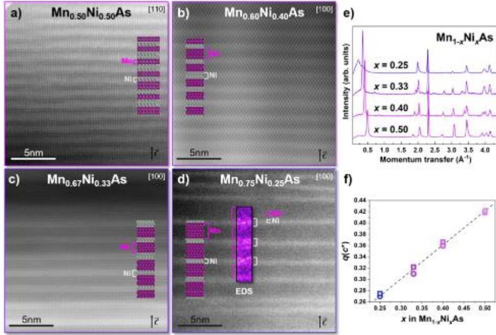
Figure 1. Experimental [110] and [100] HAADF ( \times 12M ) images of Mn_{0.50}Ni_{0.50}As , Mn_{0.60}Ni_{0.40}As , Mn_{0.67}Ni_{0.33}As , and Mn_{0.75}Ni_{0.25}As (a, b, c, and d, respectively). Brighter and darker layers correspond to NiAs and MnAs layers, respectively. Structural models extracted from 3D ED are included. An EDX spectrum is shown in panel (d), evidencing richer Mn zones (purple) and Ni zones (gray). (e) Neutron powder diffraction patterns of Mn_{0.50}Ni_{0.50}As , Mn_{0.60}Ni_{0.40}As , Mn_{0.67}Ni_{0.33}As , and Mn_{0.75}Ni_{0.25}As samples. (f) Variation of the modulation vector ( q ) vs x (circles: NPD/squares: 3D ED).
