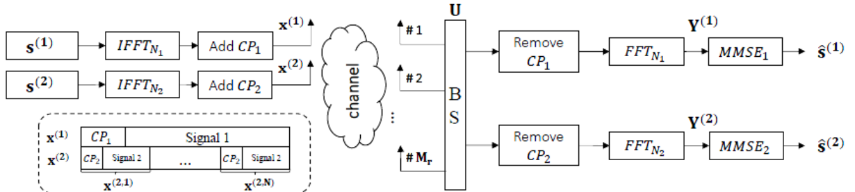
Fig. 1: System model of the massive MIMO OFDM uplink with two different numerologies: M_r receiving antennas at the BS, two single-antenna terminals, two blocks illustrate two different numerologies with OFDM of N_1 and N_2 subcarriers.
