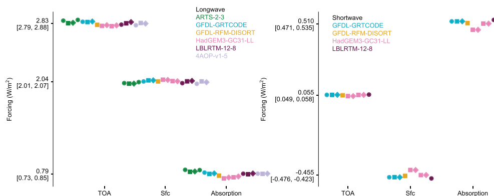
Figure 2. Global, annual mean instantaneous clear-sky radiative forcing by greenhouse gases at present day, relative to preindustrial conditions, as computed by benchmark radiative transfer models. Longwave results are on the left, shortwave results on the right, with the reference model denoted by the color. Tick labels show the mean value and range of all model results. Model names follow the RFMIP convention with contributions from SOCRATES labeled as HadGEM3 to link the results to the host climate model. Results include multiple representations of greenhouse gas changes (circles, squares, and diamonds corresponding to forcing variants 1, 2, and 3) and small variants in the treatment of some physical processes as explained in the text. All variants of the reference models agree well in longwave calculations, while SOCRATES results in the shortwave show the small but noticeable impact of different treatments of the \text{H}_2\text{O} continuum, which overlaps with absorption by other gases in the near infrared and so affects forcing by those gases.
