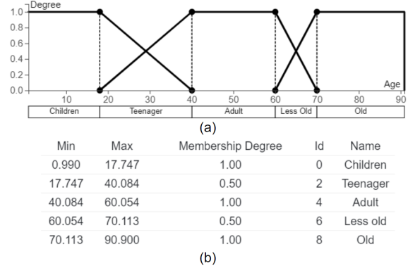
Figure 5: The age data are from 0 to 90, there are three main categories with name Chidren , Adult and Old . Meanwhile, two fuzzy categories created and they are named with Teenager and Less old .
