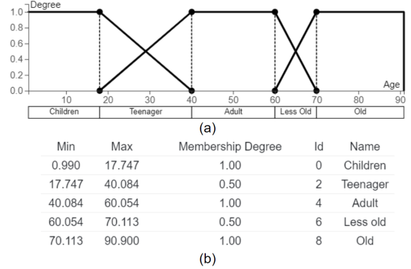
Figure 5: The age data are from 0 to 90, there are three main categories with name Chidren , Adult and Old . Meanwhile, two fuzzy categories created and they are named with Teenager and Less old .
