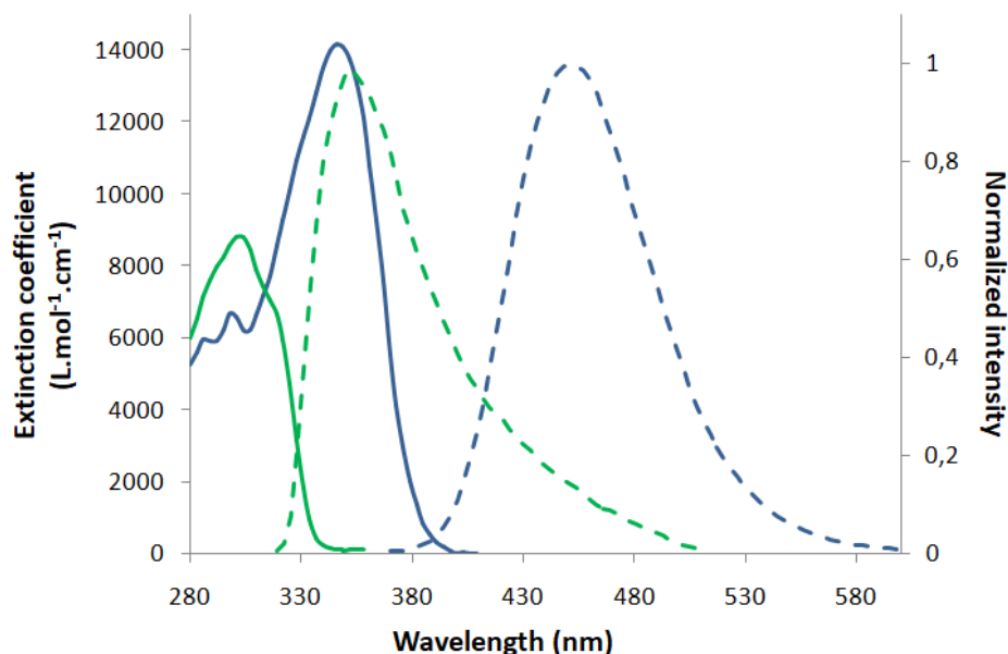
Figure 4. UV-vis absorption (continuous line) and emission (dot line) of 2 (Green) and 3 (Blue) in diluted DCM ( C = 10^{-5}\text{M} )
