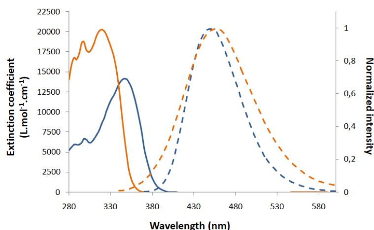
Figure 4. UV-vis absorption (continuous line) and emission (dot line) of 3 (blue) and 15 (Orange) in diluted DCM ( C = 10^{-5}\text{M} )
