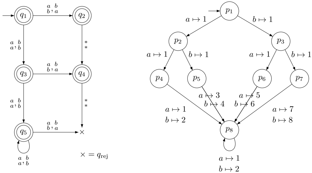
(a) Two-tape DFA. (b) Mealy automaton.
