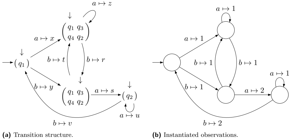
■ Figure 4 Construction of the Mealy automaton from the two-tape DFA of Figure 1b.
