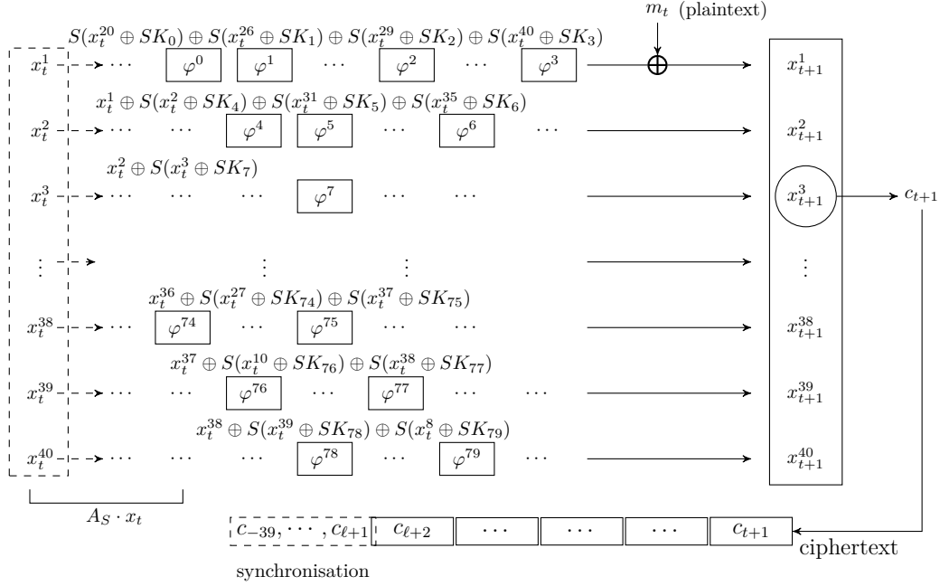
Fig. 1. The complete ciphering process of Stanislas with \varphi^i(x_t^j) = S(x_t^j \oplus SK_i) . x_t^i and x_{t+1}^i are the coefficients of the internal state at time t and time t+1 . m_t represents a plaintext symbol (4 bits), c_j the ciphertext symbols (4 bits) where c_{-39}, \dots, c_{t+2} are required for synchronisation. The equations of the lines are derived from the coefficients of the rows of the Matrix A_S .
