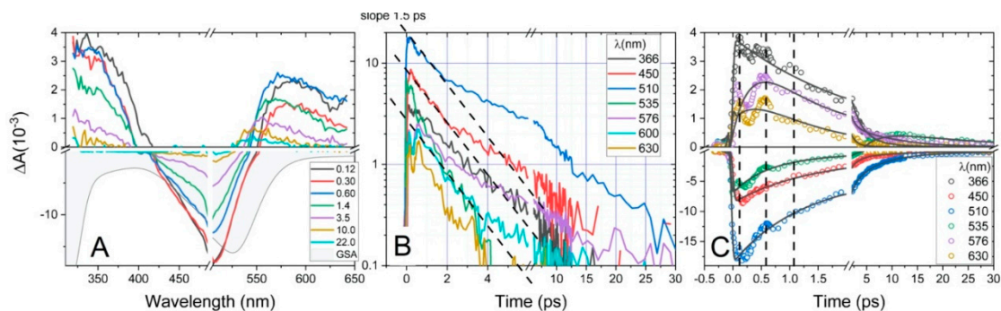
Figure 5. Femtosecond TAS data of C1 in acetonitrile (ACN) after excitation at 495 nm. (A) : Time-dependent spectra for delays in ps, as indicated in the legend. Ground state absorption (GSA) is the sign-inverted ground state absorption spectrum. Note the different scales for the positive and negative parts of \Delta A . The 480–505 nm range is disregarded due to excessive pump light scattering. (B) : Decay transients at selected wavelengths (cf. legend) plotted on a semi-log scale with a break in the time axis at 6 ps. GSB traces are sign inverted. Dashed lines are guides-to-the-eye with a 1.5 ps decay slope, highlighting that the initial fast decay of the signals is in that time range. When the signal-to-noise is large enough, an additional 10–15 ps decay emerges. (C) : Decay transients at selected wavelengths (cf. legend) plotted on a linear scale with a break in the time axis at 2.0 ps. Dashed vertical lines mark the occurrence of oscillatory maxima in the excited state absorption (ESA) with a period of \approx 0.5 ps. Solid black lines are the best fits to the data, without accounting for the oscillatory part. Note the different scales for the positive and negative parts of \Delta A . Transients are averaged over \pm 5 nm.
