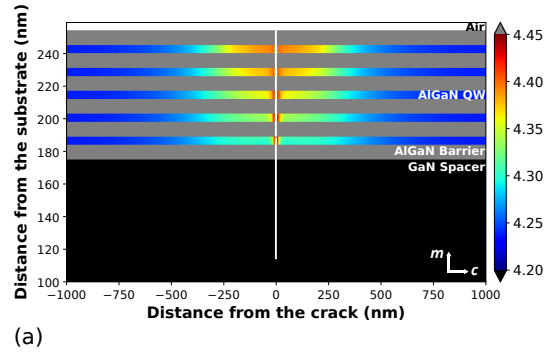
FIG. 3. (a) Mapping of the local bandgap energy in the five QWs near a crack with nextnano3 calculations. The air appears in white, the AlGaIn barriers in grey, and the GaN spacer in black. (b) Comparison between simulated and experimental energy shift as a function of the distance to the crack. The simulations correspond to the lowest energy transitions in the MQWs obtained by solving Schrödinger equation for both holes and electrons. Both (a) and (b) were simulated with an Al content of 40% in the MQWs and 60% in the barriers.
