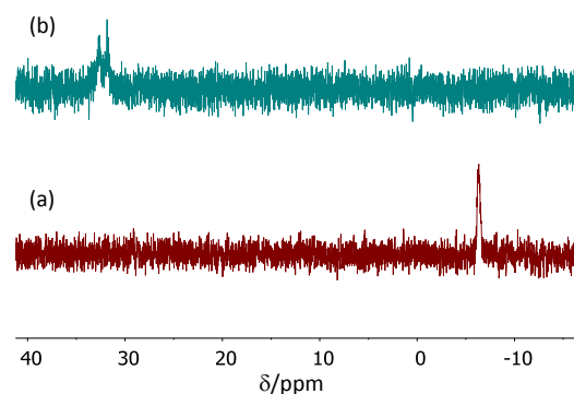
Figure 4. ^{31}\text{P} NMR spectrum for the toluene-swollen CCM 10% latex, before (a) and after (b) equilibration with a [\text{RhCl}(\text{COD})]_2 toluene solution at a P:Rh ratio of 1:1.
