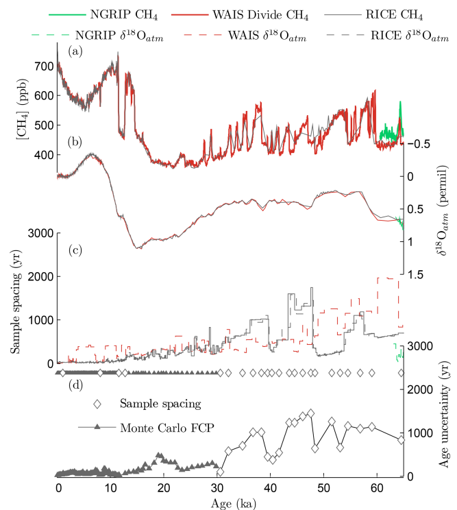
Figure 5. RICE ice core age uncertainty. (a) Methane and (b) \delta^{18}\text{O}_{\text{atm}} records from the RICE (gray), WAIS Divide (Rhodes et al., 2015; Buizert et al., 2015b) (red), and NGRIP ice cores (Baumgartner et al., 2014) (green). (c) Sample spacing for methane (solid lines) and \delta^{18}\text{O}_{\text{atm}} (dashed lines) for the various cores. (d) Gas age uncertainty, relative to WD2014, for ages determined from a Monte Carlo analysis (solid triangles) and for extended gas age control points (open diamonds).
