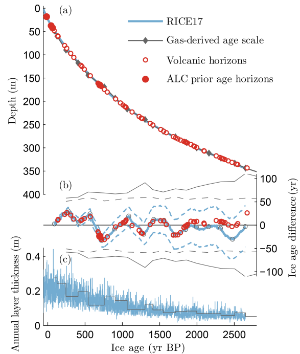
Figure 7. Comparison of the gas-derived (gray) and the annual-layer-counted ice age-scale (blue; Winstrup et al., 2019). Six absolute age markers (closed red circles) were identified, and an additional 67 volcanic horizons were cross correlated to volcanic horizons in the WAIS Divide core (plotted on WD2014 ice age-scale, open red circles; Winstrup et al., 2019). (b) Difference in ice age between the gas-derived ice age-scale and annual layer counts; positive values indicate that at the same depth the annual layer counts are older than in the gas-derived age-scale. Uncertainty estimates of the gas-derived ice age-scale (solid gray lines), the \Delta age estimate only (dashed gray lines), and the annual-layer-counted age-scale (blue dashed lines). (c) Interpretations of annual layer thickness from the gas-derived ice age-scale and annual layer interpretations.
