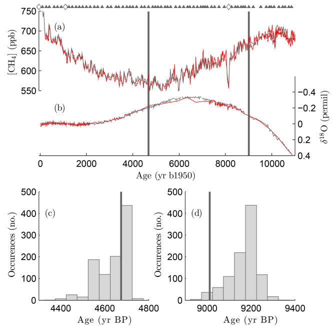
Figure 4. (a) RICE methane and (b) \delta^{18}\text{O}_{\text{atm}} records matched to those from the WAIS Divide ice core (Rhodes et al., 2015; Buizert et al., 2015b) (red lines) for the last 11.7 ka. FCPs from Monte Carlo routine are shown as solid triangles; prior constraints are shown as open diamonds. Lower panels (c, d) show the distribution of the gas ages for two particular depths, 459.05 m (4675 years BP; c) and 621.28 m (9012 years BP; d), resulting from the Monte Carlo analysis. The final age of these depths, resulting from the best realization, are shown as vertical gray lines.
