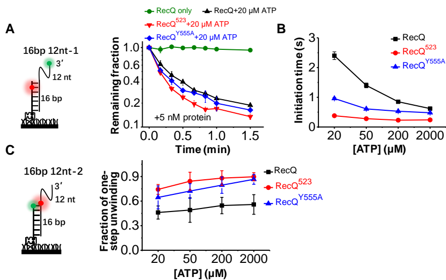
Figure 3. HRDC suppresses the duplex unwinding activity of RecQ. (A) Fractions of remaining 16bp 12nt-1 molecules on coverslip versus time after addition of 5 nM RecQ and 20 \mu M ATP. Lines are the simple connections of the individual data points by Origin 8.0. (B) The initiation time of 16bp 12nt-1 in 5 nM RecQ, RecQ 523 , and RecQ Y555A in different concentrations of ATP. (C) The fractions of 16bp 12nt-2 traces showing one-step unwinding in 5 nM RecQ, RecQ 523 , and RecQ Y555A in different concentrations of ATP.
