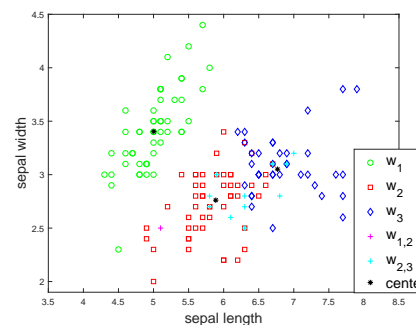
(f) Clustering results of DEC with \varphi = 0.3 .
