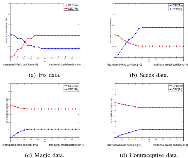
Figure 9: Clustering results of different datasets for various \varphi .
