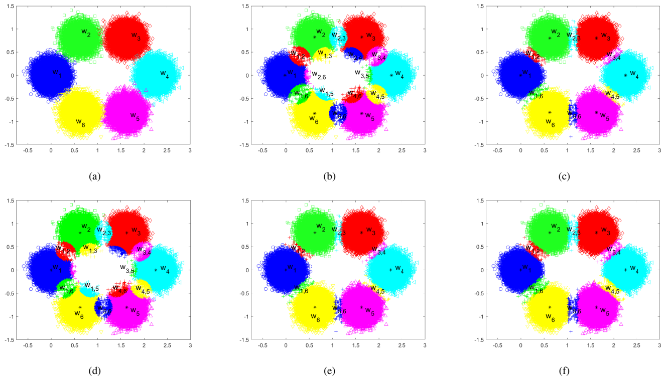
Figure 6: Clustering results of 6-class of dataset by different methods. (a) Original artificial data. (b) Clustering result of ECM ( Re = 1.13, Ri = 1.23, T = 4354.21s ). (c) Clustering result of CCM ( Re = 0, Ri = 0.30, T = 3833.51s ). (d) Clustering result of BPEC ( Re = 0.82, Ri = 1.14, T = 10534.04s ). (e) Clustering result of DEC with \varphi = 0.2 ( Re = 0, Ri = 0.21, T = 85.31s ). (f) Clustering result of DEC with \varphi = 0.3 ( Re = 0, Ri = 0.44, T = 110.90s ).
