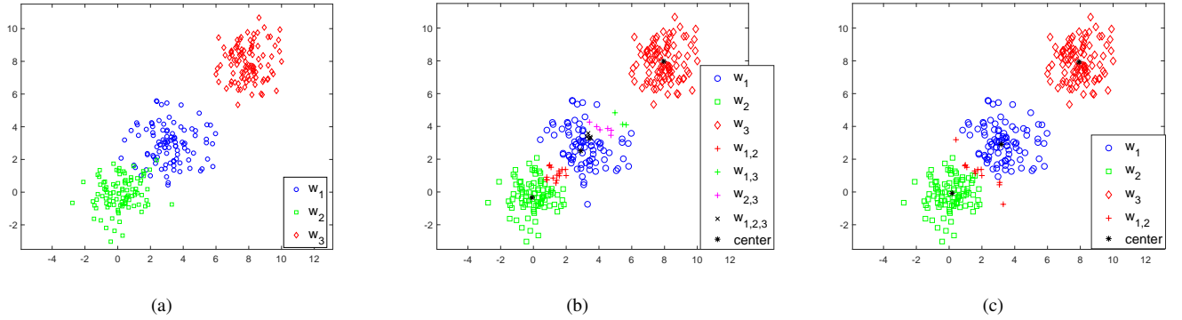
Figure 3: Clustering results of 3-class of gaussian dataset by different methods. (a) Original gaussian data. (b) Clustering result of ECM ( Re = 3.00 , Ri = 8.00 , T = 0.3011s ). (c) Clustering result of DEC ( Re = 1.00 , Ri = 4.00 , T = 0.0028s ).
