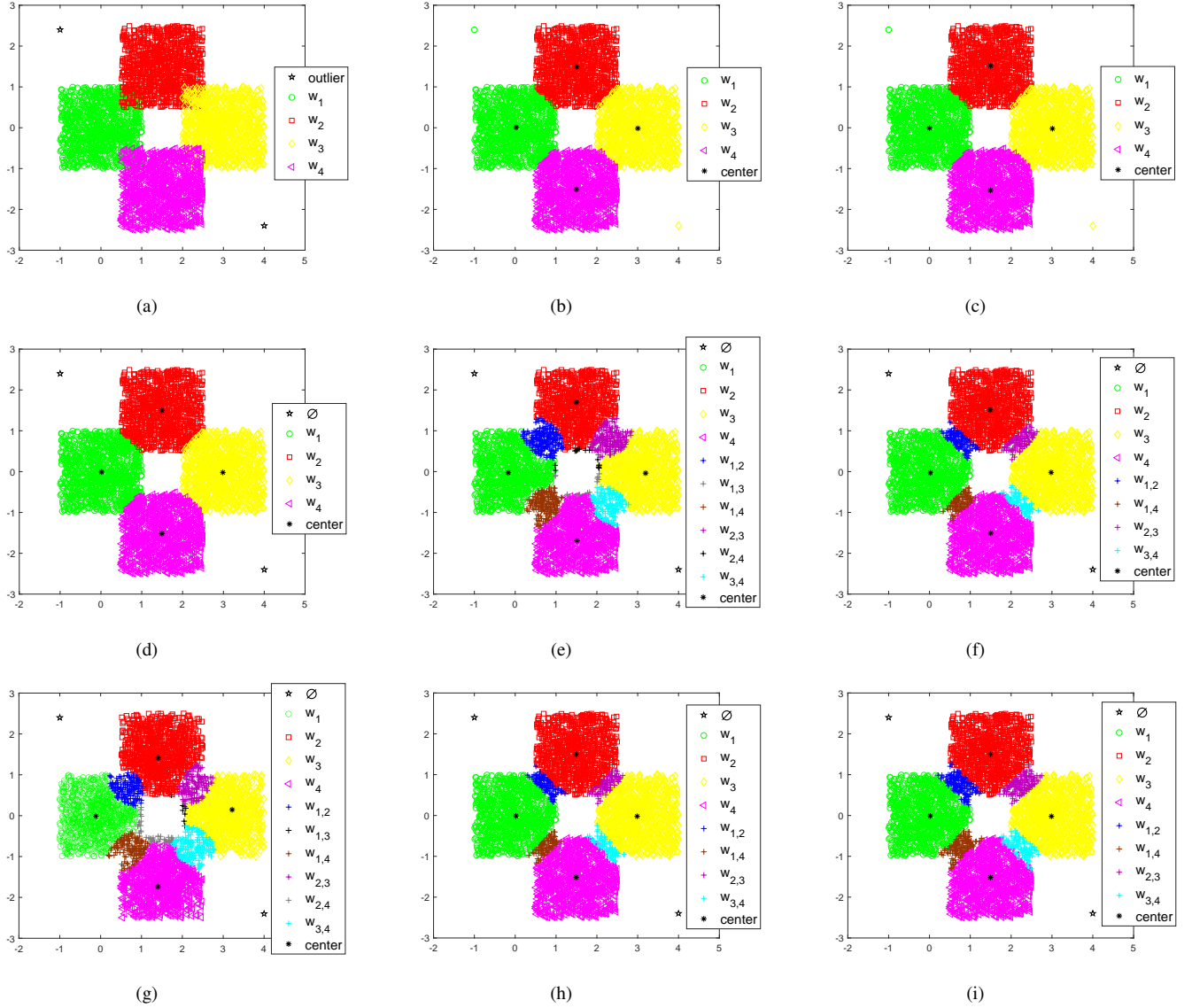
Figure 5: Clustering results of 4-class of square dataset by different methods. (a) Original square data. (b) Clustering result of C -means ( Re = 4.32, T = 0.0113s ). (c) Clustering result of FCM ( Re = 4.37, T = 0.0321s ). (d) Clustering result of NC ( Re = 4.38, T = 0.0445s ). (e) Clustering result of ECM ( Re = 0.30, Ri = 18.79, T = 6.83s ). (f) Clustering result of CCM ( Re = 1.12, Ri = 9.72, T = 5.35s ). (g) Clustering result of BPEC ( Re = 0.32, Ri = 15.17, T = 10.22s ). (h) Clustering result of DEC with \varphi = 0.2 ( Re = 1.50, Ri = 8.38, T = 0.0799s ). (i) Clustering result of DEC with \varphi = 0.3 ( Re = 0.78, Ri = 12.50, T = 0.1090s ).
