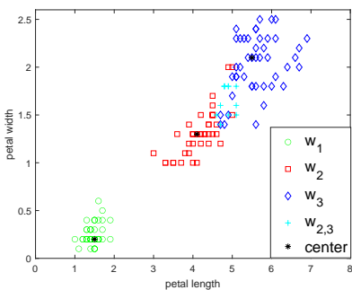
(j) Clustering results of BPEC.
