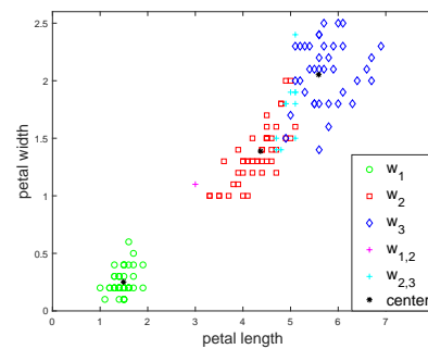
(i) Clustering results of CCM.
