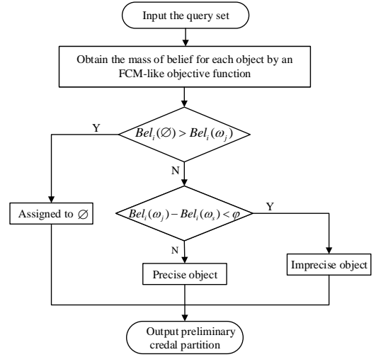
Figure 2: Flowchart of the adaptive credal partition.
