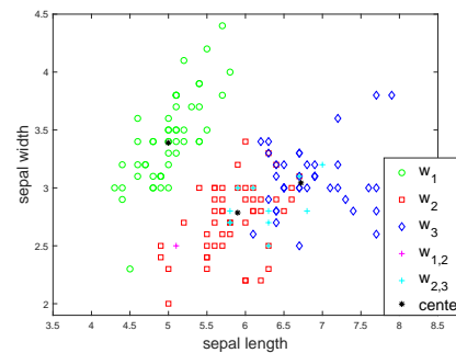
(c) Clustering results of CCM.
