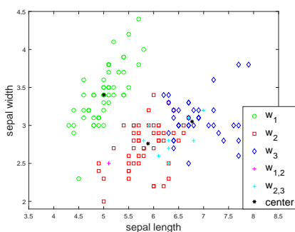
(e) Clustering results of DEC with \varphi = 0.2 .
