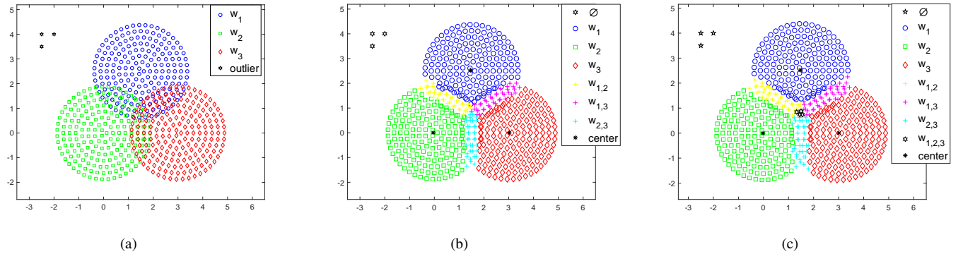
Figure 4: Clustering results of 3-class of round shape dataset by different methods. (a) Original artificial data. (b) Clustering result of CCM ( Re = 7.07 , Ri = 17.34 , T = 0.5897s ). (c) Clustering result of DEC ( Re = 4.23 , Ri = 20.81 , T = 0.0072s ).
