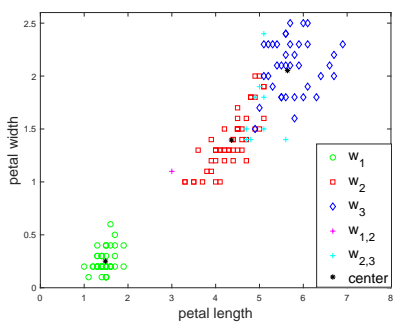
(k) Clustering results of DEC with \varphi = 0.2 .
