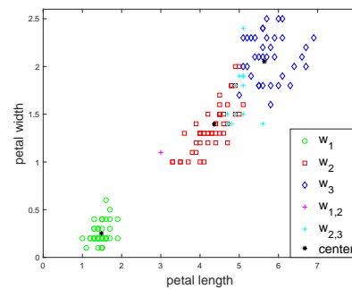
(l) Clustering results of DEC with \varphi = 0.3 .
