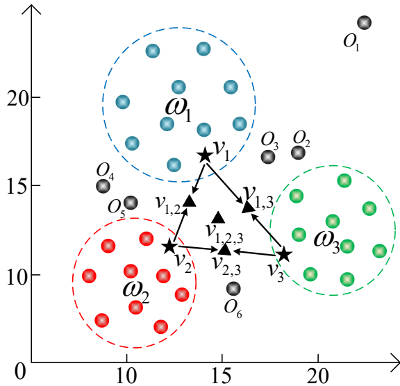
Figure 1: Illustration of the complexity in credal partition.
