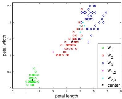
(h) Clustering results of ECM.
