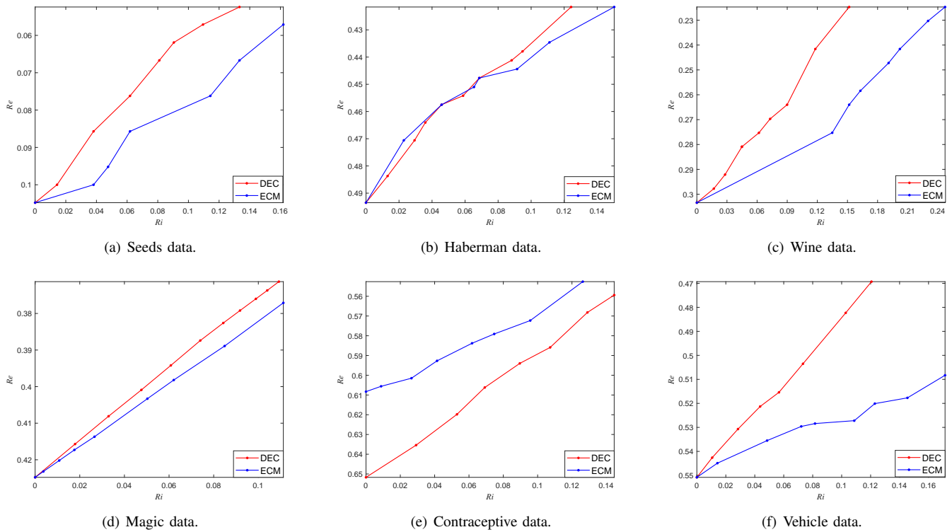
Figure 8: ROC curves for imprecision rates and error rates of ECM and DEC based on different datasets.
