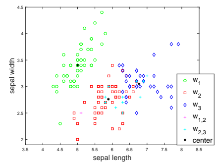
(f) Clustering results of DEC with \varphi = 0.3 .
