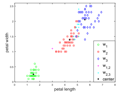
(i) Clustering results of CCM.
