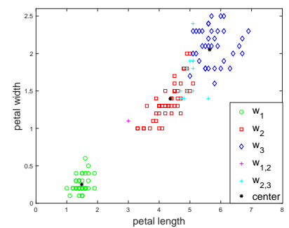
(l) Clustering results of DEC with \varphi = 0.3 .
