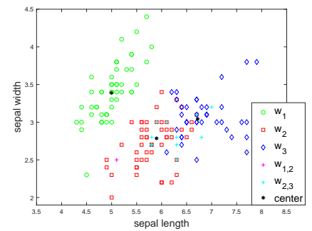
(c) Clustering results of CCM.
