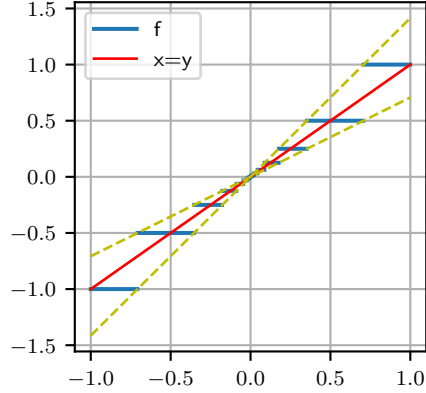
Figure 10: Example of a non-continuous function f with values in \{(\frac{1}{2})^n \mid n \in \mathbb{N}\} , approximating the identity function. However, this function is not differentiable because the difference quotient does not converge but instead oscillates between two values.
