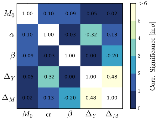
Fig. 7. Correlation matrix between the coefficients of the 4-parameter standardization (SALT2 .4 x_1 and c , along with \mathcal{P}_Y and \mathcal{P}_{HM} ). The values within the matrix are the correlation coefficients. The color of the matrix elements represent the significance of this correlation coefficient.
