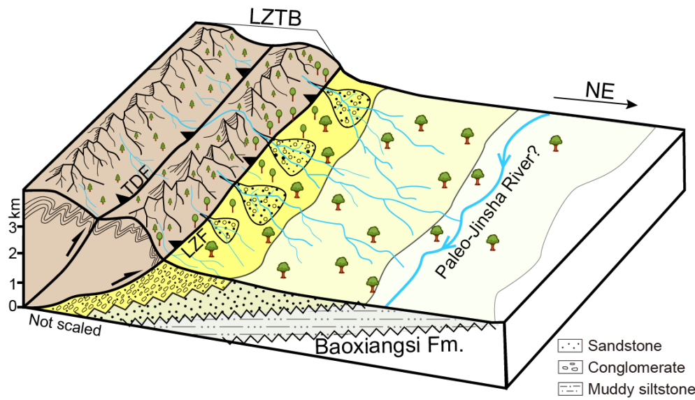
Fig.8 Cartoon showing middle Eocene source-to-sink relationship between the LZTB and syn-tectonic sediments of Baoxiangsi Fm. ( E_2b ) in the Jiachuan basin. Topographic relief was produced by the activity of the LZTB during ~50-39 Ma, resulting in a high vegetation diversity from the mountains to relatively low-elevation basin recorded by pollen grains (Wu et al., 2018).
