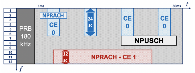
Fig. 1: NB-IoT - Uplink Frame
