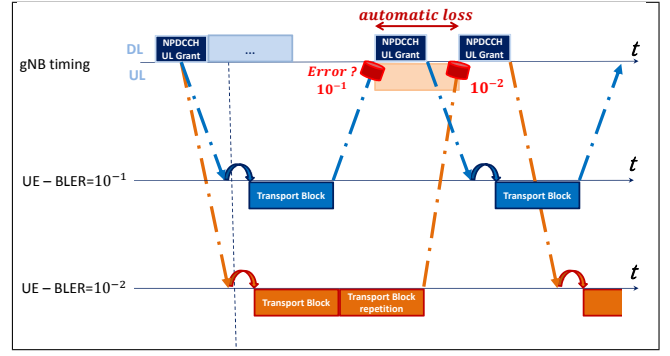
Fig. 5: Error free HARQ process for 2 different BLER selections.
