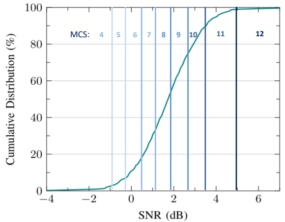
Fig. 8: SNR distribution for uplink in GEO case (3GPP assumptions). Modulation and Coding Scheme (MCS) indexes are shown for a BLER target of 10^{-1} and multi-tone 45 kHz modulation. Thresholds have been derived from Figure 7.
