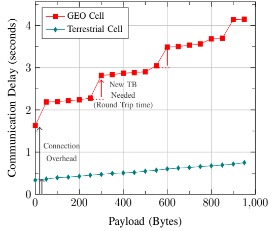
Fig. 9: Delay of communications from first connection attempt to last payload bytes sent, depending on payload and cell type. The differences are due to coverage and round trip delay. Data plotted for BLER = 10^{-1} .
