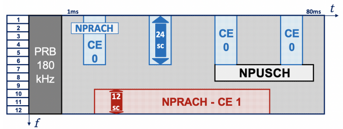
Fig. 1: NB-IoT - Uplink Frame
