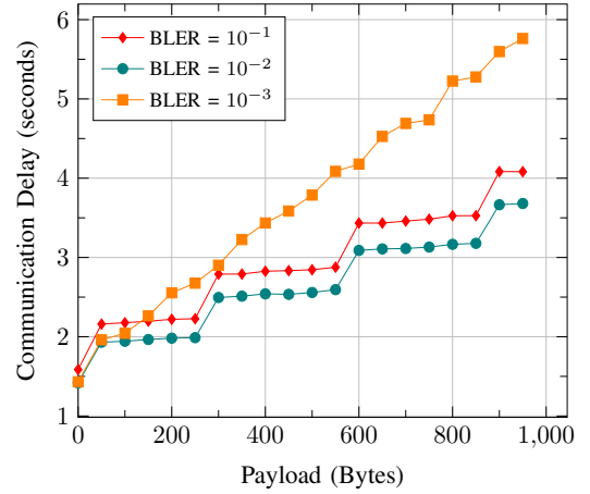
Fig. 10: Delay of communications depending on robustness (BLER) and payload. The optimum configuration for latency is found around a BLER of 10^{-2} . A value all the more interesting knowing that the targeted BLER in terrestrial deployment is 10^{-1} .
