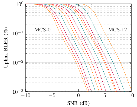
Fig. 7: Uplink Block Error Rate curves depending on Signal to Noise Ratio. Modulation and Coding Scheme (MCS) is varying from index 0 to index 12 (multi-tone transmission).
