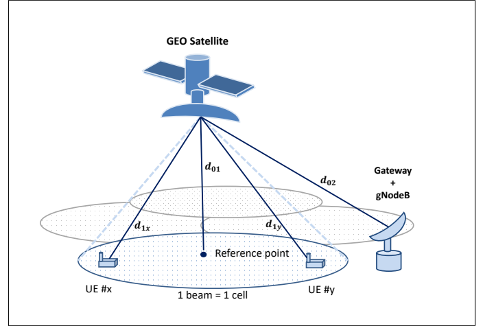
Fig. 2: Transparent GEO satellite scenario
