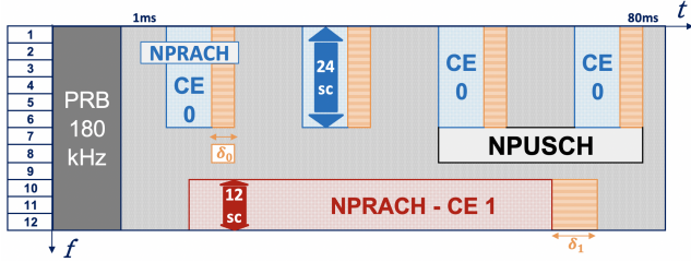
Fig. 4: Differential delay impact on UL Frame
