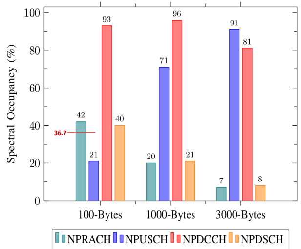
Fig. 13: Occupancy of the spectral resources when the cell reaches its maximum utilization. Depending on the payload size the resource starvation does not occur on the same channel.
