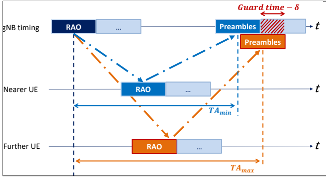
Fig. 3: Differential delay effect
