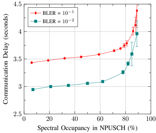
Fig. 11: Delay of communications from first connection attempt to last payload bytes sent, depending on spectral occupancy and BLER.
