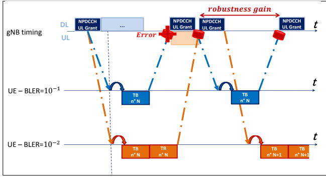
Fig. 6: BLER impact on the HARQ process in the case of an error on the UE with the least robust communication.
