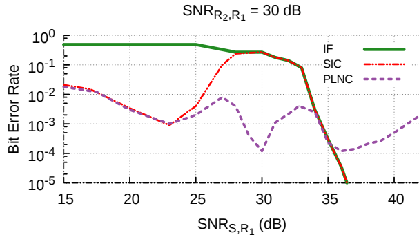
Figure 3: Error Rate at R_1 with different values of SNR_{S,R_1}
