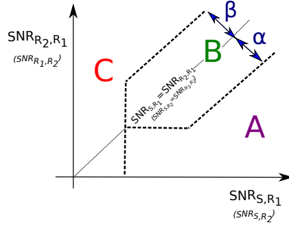
Figure 4: Three decoding strategies at R_1 depending on the intra-diamond channel (IDC)
