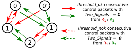
Figure 6: Source rate adaptive protocol state machine
