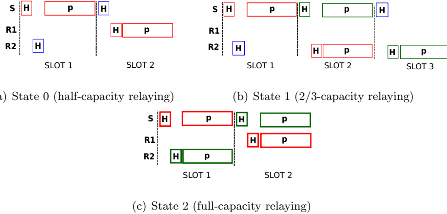
Figure 5: COLiDeR introduces 3 scheduling policies: the traditional half-capacity one-path relaying (5(a)); 2/3-capacity two-path relaying (5(b)); and full-capacity two-path relaying (5(c)).
