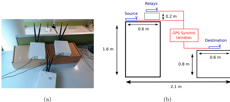
Figure 2: USRP testbed used for implementing and evaluating diamond-based relaying.
