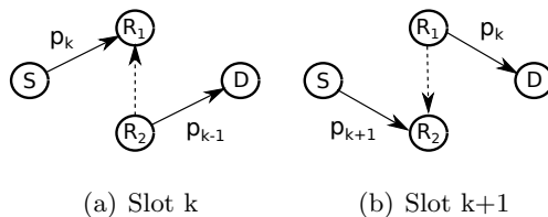
Figure 1: Two-path relaying. The source, S , transmits on every slot, alternating between the two relays, R_1 and R_2 . When a relay is receiving from the source, the other transmits to the destination, jointly creating the equivalent of a single full-duplex relay.
