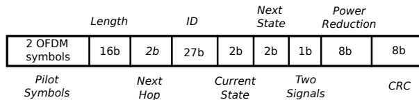
Figure 7: Control Packet Format
