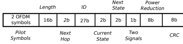
Figure 7: Control Packet Format
