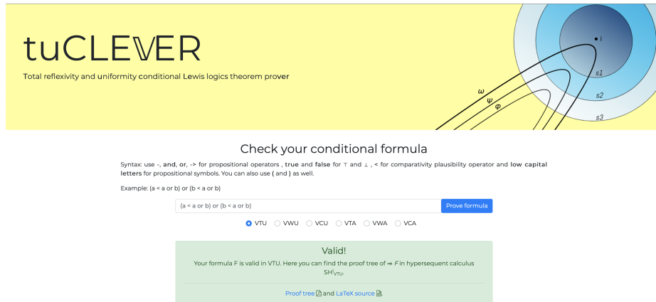
Fig. 3. When the formula is valid, tuCLEVER computes both a pdf containing the derivation found by the prover and its \text{L}^{\text{A}}\text{T}_{\text{E}}\text{X} source file.
