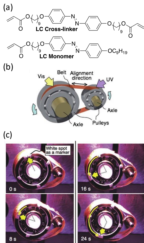
Figure 65: (a) Structures of the monomer and of the cross-linking agent. (b) Scheme of the experimental setup of the light-fuelled motor. A LC film is placed around two pulleys and irradiated by UV on one side and visible light on the other. Contraction of the film followed by its expansion allows the ribbon to move. (c) Pictures of the rotation of the motor overtime, the white spot can be used as a marker to follow the rotational motion. Parts (b) and (c) are adapted with permission from reference 897 , Copyright 2008 John Wiley and Sons.
