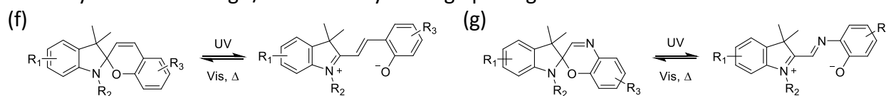
Figure 1: Chemical structures of photoisomerizable (a) azobenzene, (b) stilbene, (c) hydrazone, (d) diarylethene, (e) fulgide (labile hydrogen highlighted in red), (f) spiropyran and (g) spirooxazine.
