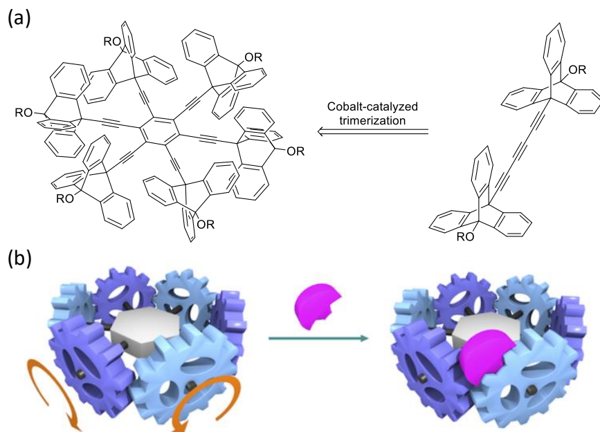
Figure 108: Design principle and realization of an intramolecular bevel gear. (a) Molecular structure and synthetic strategy to access the sextuple gear with six triptycene gears attached to the central benzene ring through ethynyl linkers. (b) Schematic representation of the gearing process and of its control by locking the triptycene rotation when complexed to bulky RuCp*. Adapted with permission from reference 1117 , Copyright 2017 American Chemical Society.
