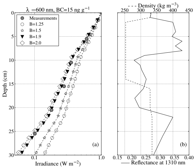
Fig. 2. Measurements conducted at Col de Porte (29 February 2012). (a) The measured irradiance profile at \lambda_{k_e} = 600 nm is shown with the optimal modelled profile symbolized by dark inverted triangles. The other profiles have been calculated for various values of B and incident flux equal to the optimal I_0(600nm) . All profiles are normalized at the surface. (b) Vertical profiles of density and reflectance at 1310 nm used to compute the irradiance profiles in (a).
