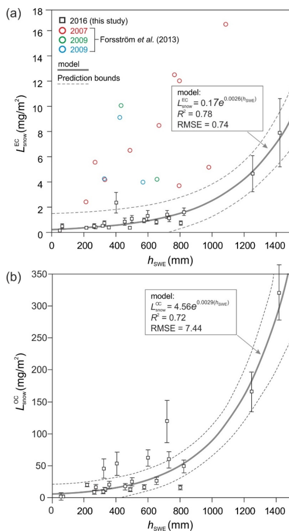
Fig. 6. Scatterplot of (a) L_{\text{snow}}^{\text{EC}} and (b) L_{\text{snow}}^{\text{OC}} against h_{\text{SWE}} based on measurements from Svalbard glacier snowpits from the April 2016 survey. The error bars are \pm 1\sigma , and take into account uncertainties in h_{\text{SWE}} , C_{\text{snow}}^{\text{EC}} , and C_{\text{snow}}^{\text{OC}} . An exponential model, shown with 95% confidence bounds on predictions, was fitted by nonlinear least-squares regression, inversely weighted against data errors. In panel (a), data from earlier surveys by Forsström et al. (2009, 2013) are displayed for comparison.
