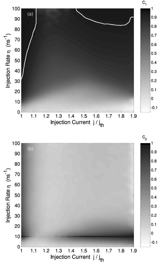
FIG. 12. Synchronization regions in the parameter space (injection current, optical coupling rate). (a) The value of C_1 is plotted. The white line corresponds to the threshold injection rate above which C_1 is larger than 0.95. For 1.15j_{th} < j < 1.4j_{th} approximately, the threshold injection rate is larger than 100 \text{ ns}^{-1} (b) The value of C_2 is plotted. \Delta\omega=0 , \gamma_s=0 , all other parameters as in Fig. 4.
