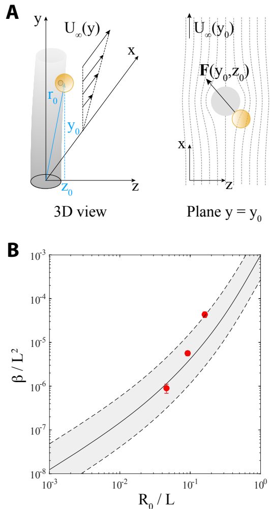
FIG. 4. (A) Sketch of the physical situation for a particle/fiber contact interaction. Left panel – 3D view. Right panel – Top view in the plane y = y_0 . U_\infty denotes the flow magnitude far away from the fiber. (B) Red disks correspond to the experimental values of \beta (see Table 1) divided by L^2 as a function of the normalized particle size R_0/L . The solid line corresponds to the theoretical predictions of the contact model, with a = 50 \mu\text{m} , L = 435 \mu\text{m} , E = 2.7 \text{ MPa} and \eta = 119.7 \text{ mPa}\cdot\text{s} . The dashed lines estimate the model prediction limits taking \pm 5\% variations in L and variations of E and \eta within their experimental errors.
