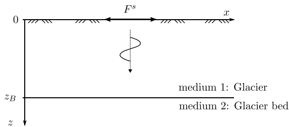
Figure 1. Schematic representation of the seismic shear wave traveling downward in a two-layer one-dimensional system. Medium 1 represents the ice body (assumed as an elastic medium) and medium 2 is the porous basement (assumed as a poroelastic medium).
