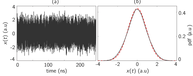
Fig. 2. (a) Time series of x(t) , (b) probability density function (gray line) of x(t) and a theoretical Gaussian distribution (red dashed line). The parameters are \tau = 25 ps, \theta = 10 \mu s, T_{i=1,2} = 30 ns, \beta_{i|i=1,2} = 5 , \phi_{0i|i=1,2} = -\pi/4 , \omega_2 = 2\omega_1 = 2 , and time step \Delta t = 5 ps.
