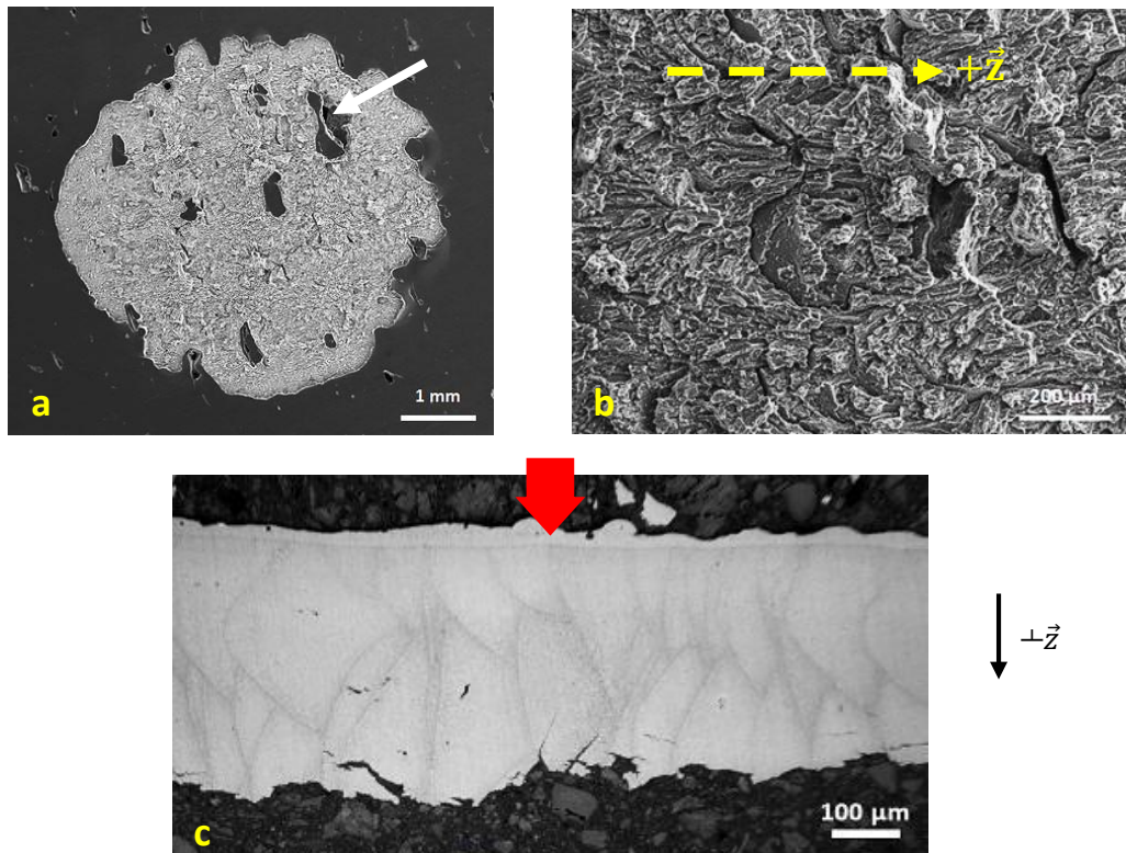
Fig. 12. Scanning Electron Micrographs of the spall crater in sample P2-XY-500-1 shocked along the normal to the building direction (a, b), and optical micrograph of a cross section of the sample (c). The white arrow points to a lack of fusion. Fracture is mainly intrapool, except for some interpool cracks at boundaries of propitious location and orientation.
