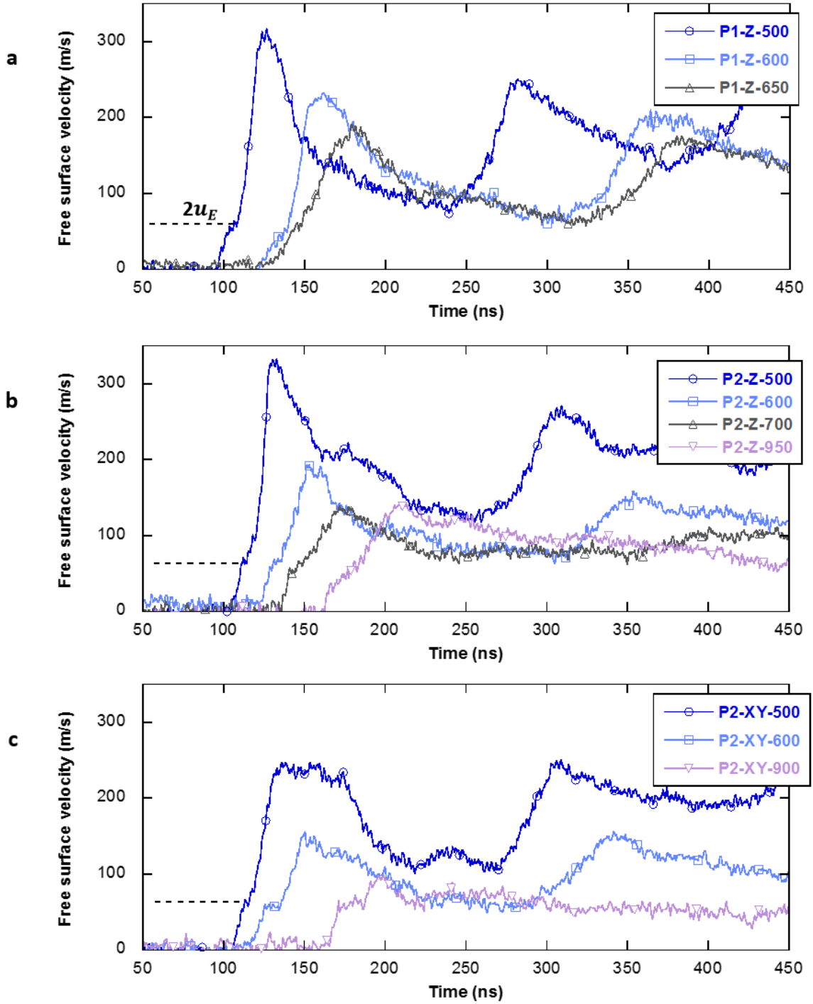
Fig. 4. Free surface velocity profiles of (a) P1 samples loaded along Z axis, (b) P2 samples irradiated along Z axis and (c) P2 samples irradiated orthogonally to Z axis. Samples are referenced with their thickness in \mu\text{m} .
