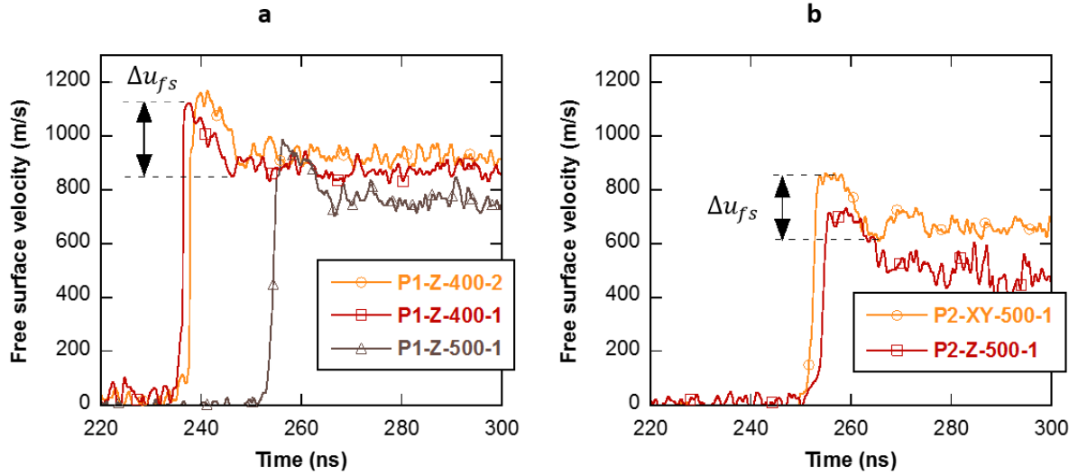
Fig. 7. Free surface velocity profiles recorded in (a) P1 samples, (b) P2 samples. Shots are referenced with the direction of shock application and sample thickness in \mu\text{m} .
