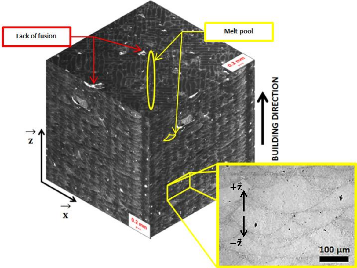
Fig. 1. 3D Reconstruction of optical micrographs showing the typical microstructure of SLM-produced AlSi10Mg alloy (after polishing, without etching). Melt pools are visible in their length on the top view, while the cube sides show them in their height (along the z axis) and width (along the x and y axes). The cube side length is 5.5 mm.
