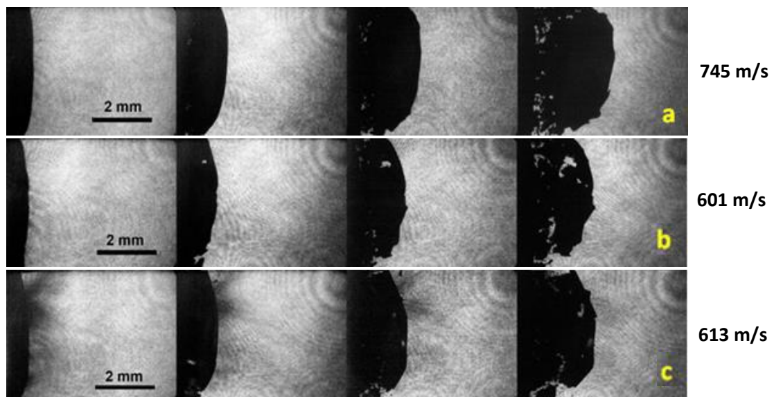
Fig. 8. Transverse shadowgraphs recorded at 1\mu\text{s} , 2\mu\text{s} , 3\mu\text{s} and 4\mu\text{s} from left to right, in (a) P1-Z, (b) P2-Z and (c) P2-XY samples with the mean velocity of the main spalled layer.
