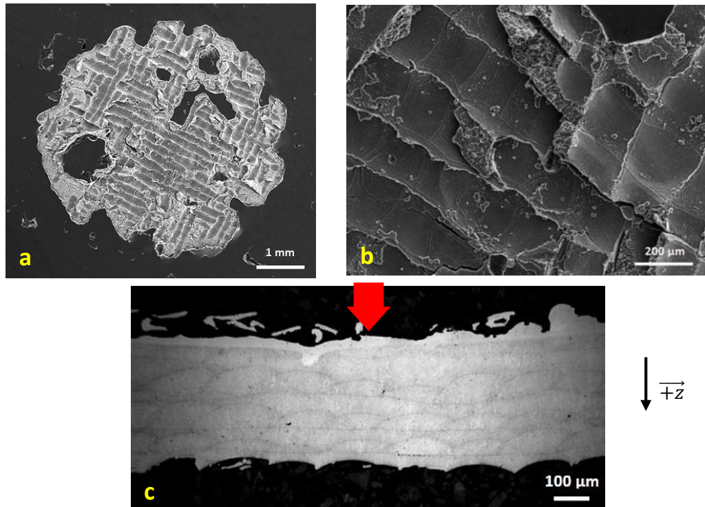
Fig. 11. Scanning Electron Micrographs of the spall crater in sample P2-Z-500-1 shocked along the +z axis (a, b), and optical micrograph of a cross section of the sample (c).
