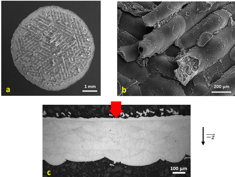
Fig. 9. Scanning Electron Micrographs of the spall crater in sample P1-Z-500-1 shocked along the -Z axis (a, b), and optical micrograph of a cross section of the sample (c).
