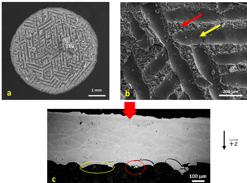
Fig. 10. Scanning Electron Micrographs of the spall crater in sample P1-Z-500-2 shocked along the +Z axis (a, b), and optical micrograph of a cross section of the sample (c). Arrows and circles show both intrapool (red) and interpool fracture (yellow).
