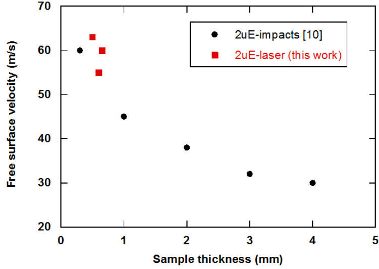
Fig. 6. Velocity 2u_E measured in SLM-produced AlSi10Mg samples of increasing thickness: red squares refer to laser-shock loading of the P1 alloy, while black circles result from plate impacts [10].
