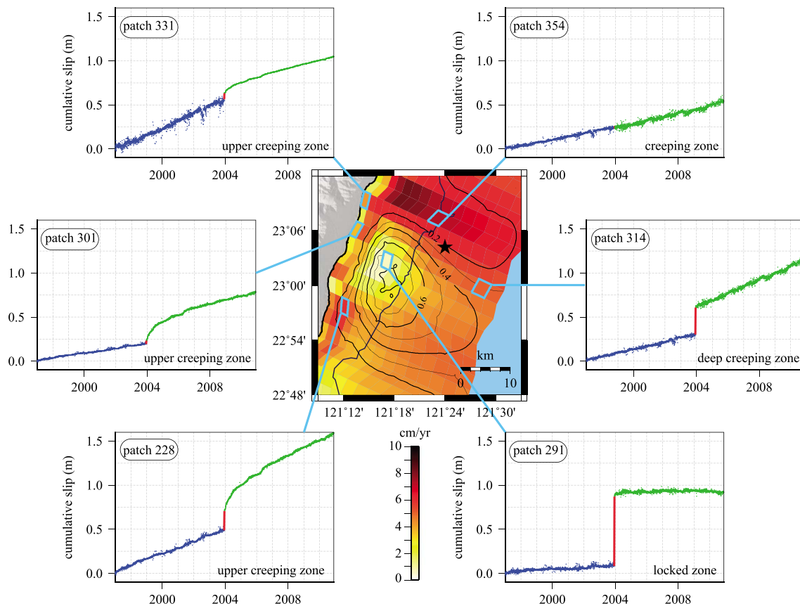
Figure 15. Slip at depth through time obtained from combining PCAIM inversions of preseismic and postseismic period and coseismic slip due to the Chengkung earthquake. Map view shows a close-up view of the secular slip rate distribution over the whole study period (see Figure 7a for location), with contour lines of the coseismic slip model (black lines) and epicenter (star) of the 2003 Chengkung earthquake. Graphs around the map view show the time evolution of slip at six patches along the direction of the slip vector predicted by the block motion of the Coastal Range relative to the Central Range. Patch 331, 301, and 228 sample the upper creeping zone. Patch 291 is characteristic of the zone which was locked before the Chengkung earthquake, slipped during the event, and relocked immediately after. Patches 314 and 354 illustrate the behavior of the deeper fault portion which is most poorly resolved.
