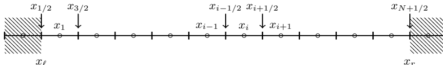
Figure 2: Colocated mesh
