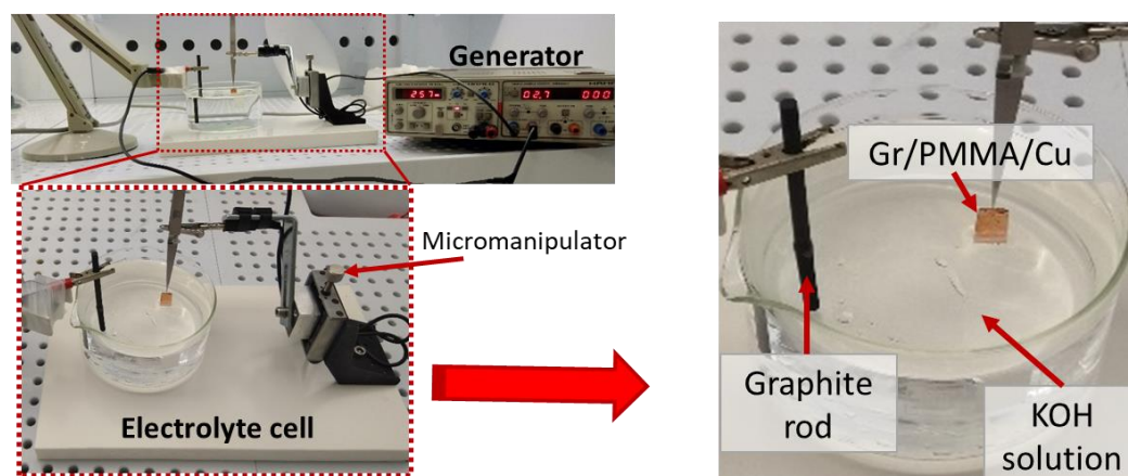
Fig S5: Experimental setup for electrochemical delamination of graphene.
