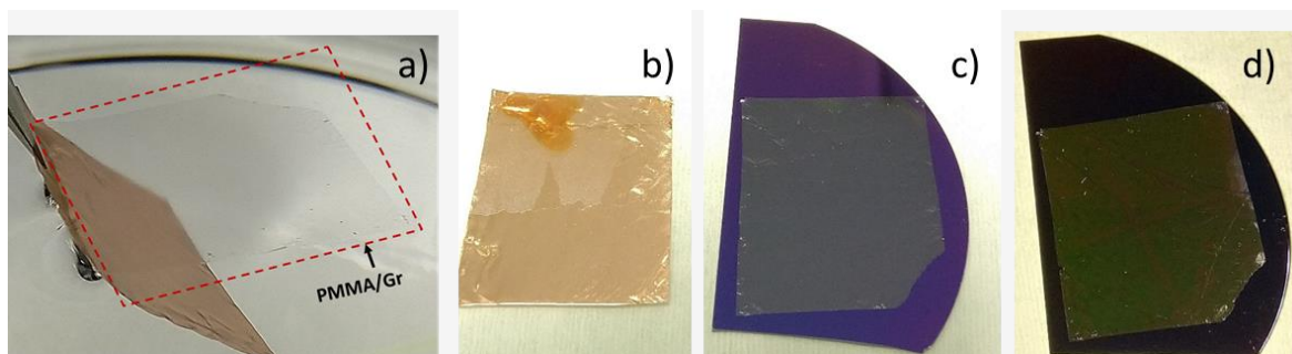
Fig S6-II: transfer using optimal parameters (2.7 V, 42 mmol/L) showing the PMMA/Graphene film (a) during the separation from copper (b) on copper (c) on SiO 2 before annealing (d) on SiO 2 after annealing.
