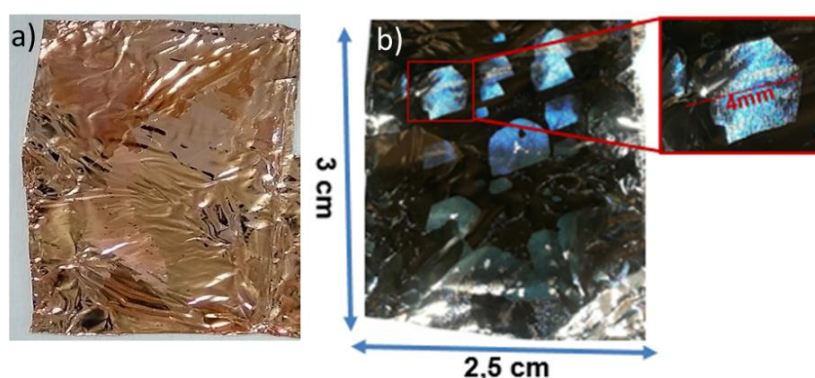
Fig S2: Unfolded copper pocket, inside face, after growing graphene monocrystals (a) optical image of the Cu foil without flashlight and (b) with flashlight that helps to visualize the large crystals grown on the top.
