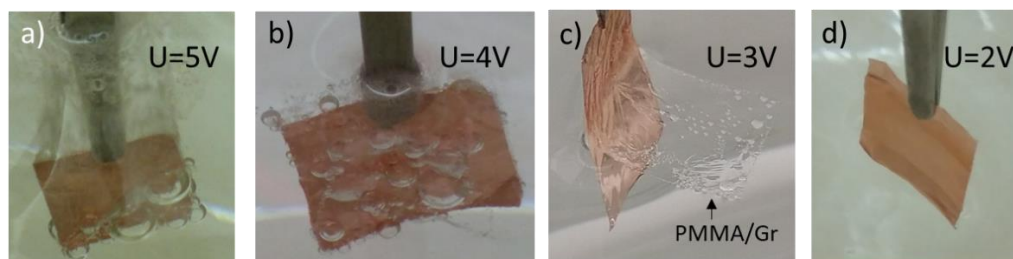
Fig S6-I: Effect of the applied voltage on H 2 bubbles generated during transfer (a) vigorous flow for 5V (b) fewer bubbles for 4V (c) almost no bubbles for 3V and (d) no bubbles but no reaction at 2V.
