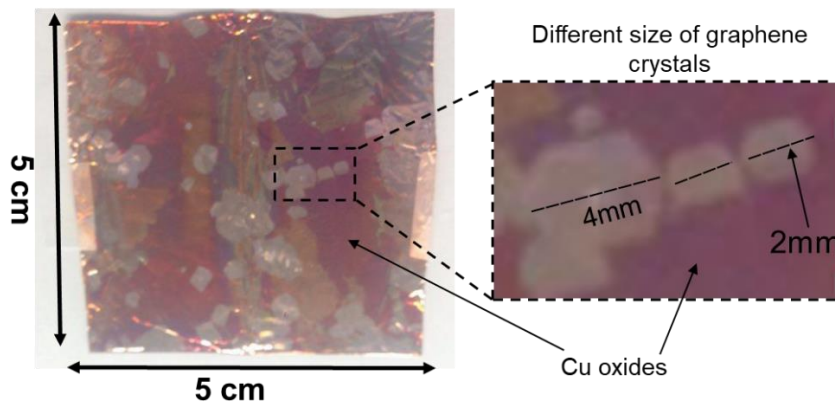
Fig S3 : Optical image of graphene nanocrystals on copper foil after post-growth annealing. The resulting oxidation of copper makes individual crystals visible by eyes.
