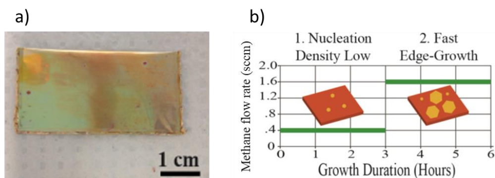
Fig S1: (a) Optical image of the copper foil folded in half, the remaining three sides being carefully crimped to obtain an enclosed pocket (b) Illustration of the two-step growth process of the graphene monocrystals.
