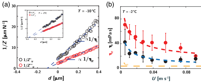
FIG. 3. Complex rheology. (a) Inverse of the mechanical impedance 1/Z'_N and 1/Z''_N as a function of the retract distance d for two distinct temperatures. We observe a linear behavior for both impedances, typical of a viscoelastic fluid. (b) Evolution of the real and imaginary parts of the viscosity as a function of the shearing speed U . The dashed lines correspond to a fit \eta_{R,I} \propto U^{-\alpha} with \alpha = 0.5 . The yellow line indicates the viscosity of supercooled water \eta_{\text{WS}} .
