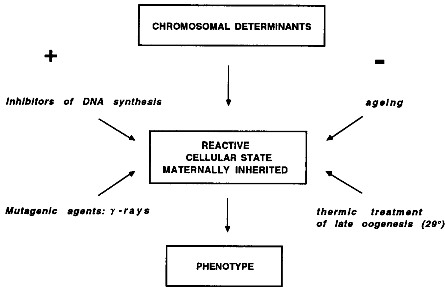
FIGURE 1.—Schematic presentation of the genetic behavior of the reactivity level. Until now the phenotype was only the frequency of transposition of I factor.
