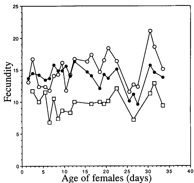
FIGURE 4.—Fecundity of irradiated flies of the A series (○), the B series (●) and the C series (□). Statistical analysis of these data is presented in Table 2. Fecundity is expressed in mean number of eggs laid by female by 24 hours.
