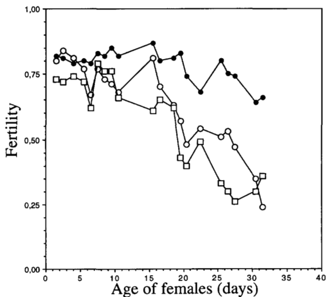
FIGURE 5.—Fertility of irradiated flies of the A series (○), the B series (●) and the C series (□). Statistical analysis of these data are presented in Table 2.
