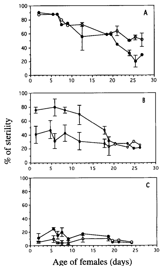
FIGURE 3.—Changes in reactivity induced by 40-Gy irradiation of females sharing the same nuclear genotype but with different reactivity levels; irradiation was applied at pupal stage. Control series (○), irradiated series (●) (A) Strongly reactive flies. (B) Flies with medium reactive level. (C) Weakly reactive flies.
