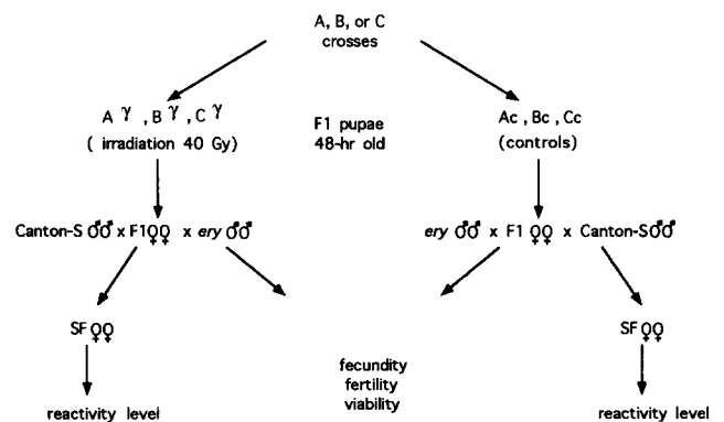
FIGURE 2.—Experimental scheme used to compare sensitivity to gamma rays of flies bearing the same genetic background but with different reactivity levels. A cross is: seF8 females × ery males; B cross is: seF8LG females × ery males; C cross is: ery females × seF8 males.
