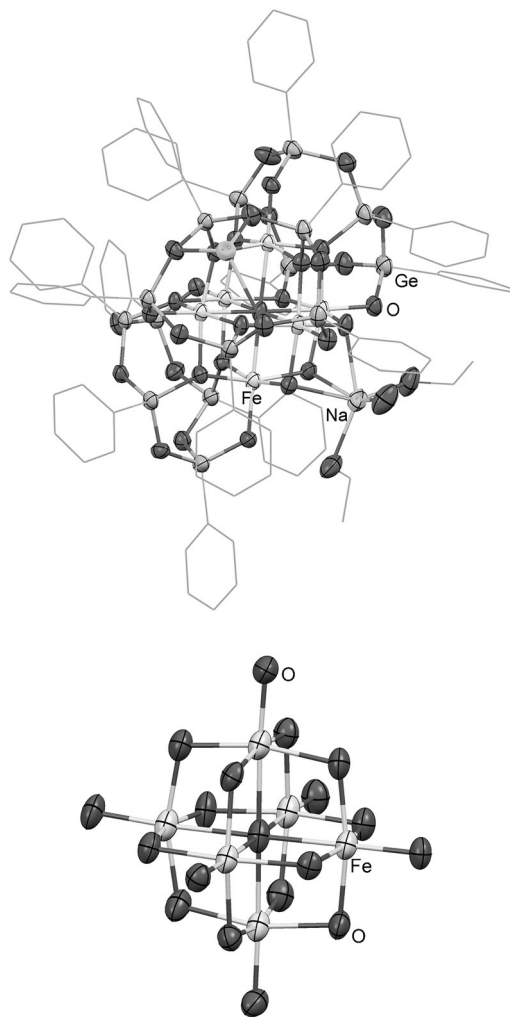
Figure 1. Top: Molecular structure of 1 . Bottom: The structure of Fe 6 O 19 core of 1 . Full color version is given in ESI (Figures S1,S2).
