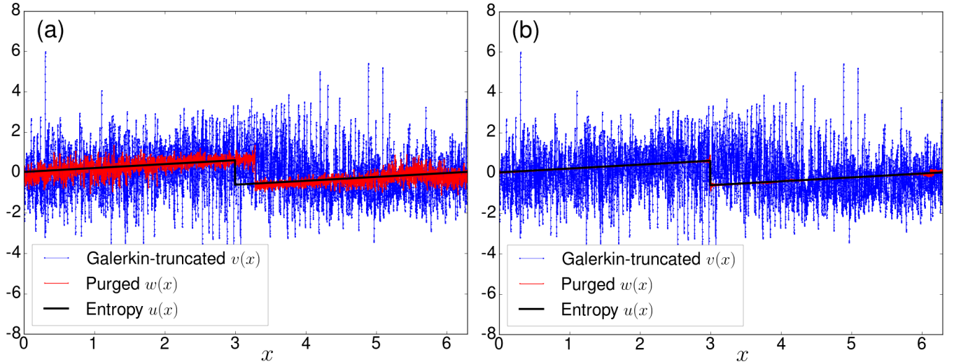
FIG. 2. Representative plots, for K_G = 1000 , of the Galerkin-truncated v (blue), the entropy u (black), and the purged w (red) solutions of the Burgers equation at t = 5.0 for (a) \alpha = 0.6 , \beta = 0.4 and (b) \alpha = \beta = 0.8 . In panel (b), the purged and entropy solutions are quite close to being identical. A movie of the full evolution in time of the solutions shown in panel (b) is available [34].
