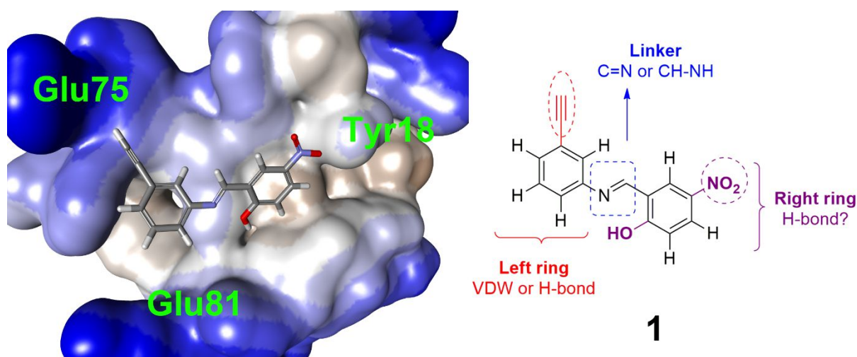
Figure 2. The docking model showing the interaction of the hit compound 1 with E. coli NusB (PDB:3D3B) with the hydrophilicity of NusB surface is colored in blue (left) and the modification plan of the hit compound 1 (right).
