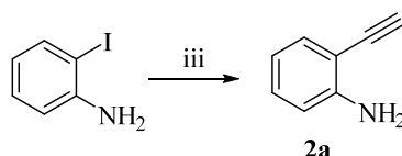
Scheme 1. Synthesis of a) the target compounds 1-19 , 20-35 and b) intermediate 2a
