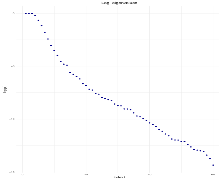
Figure 3: Decay of the base learner eigenvalues in logarithmic scale - only the 60 largest eigenvalues are plotted due to numerical instability for smaller ones.
