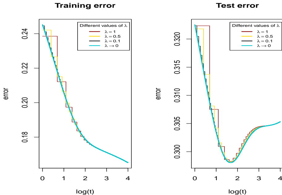
Figure 2: Training and test error of the predictors \hat{F}_t(\cdot) and \hat{F}_{[t/\lambda]}^\lambda(\cdot) for different values of \lambda .
