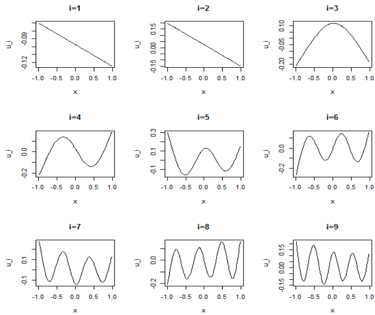
Figure 5: First eigenvectors of the linear base learner interpreted as signal.
