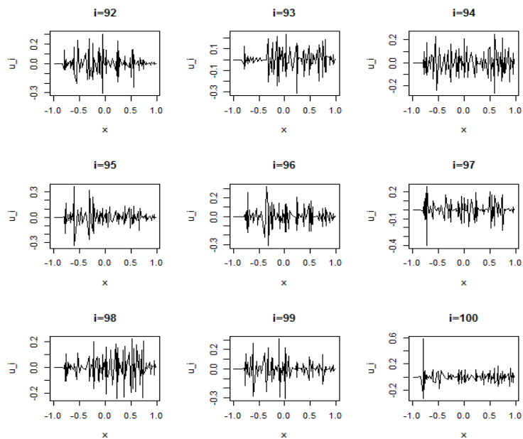
Figure 6: Last eigenvectors of the linear base learner interpreted as noise.
