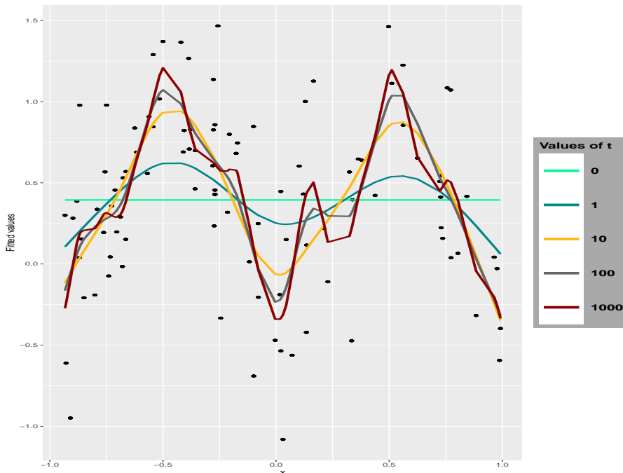
Figure 1: Output of the L^2 -Boosting algorithm in the vanishing learning rate asymptotic with input (Y_i, X_i)_{1 \leq i \leq 100} generated from model (26) at different values of t . The black dots represent the observed data set (Y_i, X_i)_{1 \leq i \leq 100} .
