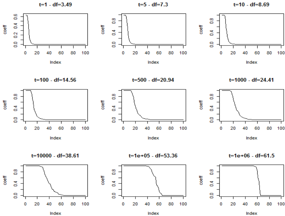
Figure 4: Coefficient appearing in Equation (27), the interpretation of the boosting linear operator as a smoothed projection.
