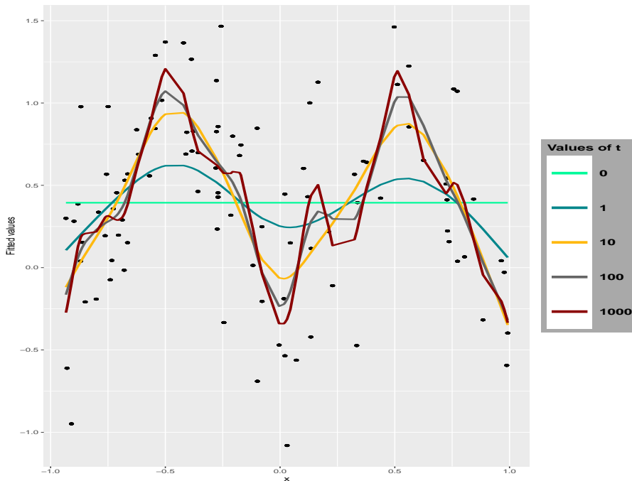
Figure 1: Output of the L^2 -Boosting algorithm in the vanishing learning rate asymptotic with input (Y_i, X_i)_{1 \leq i \leq 100} generated from model (26) at different values of t . The black dots represent the observed data set (Y_i, X_i)_{1 \leq i \leq 100} .
