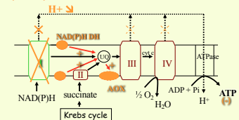
Respiratory chain of CMS II mutant of Nicotiana sylvestris
