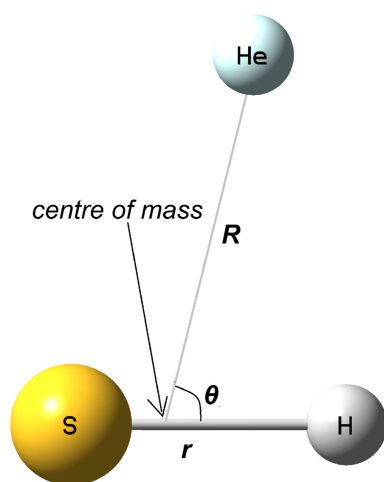
FIG. 1. Body-fixed Jacobi coordinates of the SH^- -He collisional complex.
