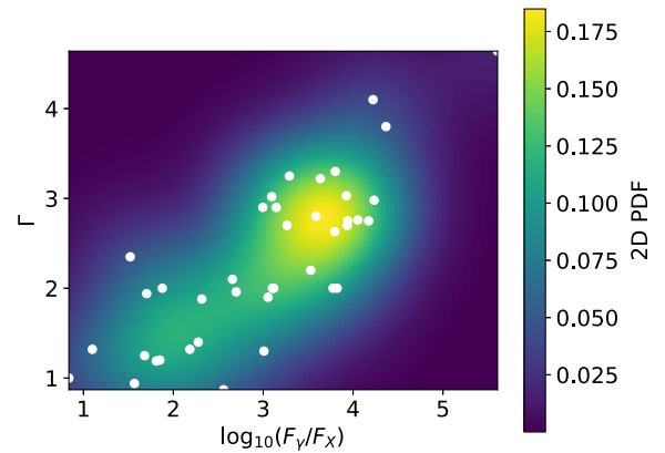
FIG. 2. KDE 2D joint PDF (colored background) of \log_{10}(F_\gamma/F_X) and x-ray spectral index \Gamma from the 40 x-ray observed MSPs having a \gamma -ray counterpart. Original data from [27] are shown by the white dots.
